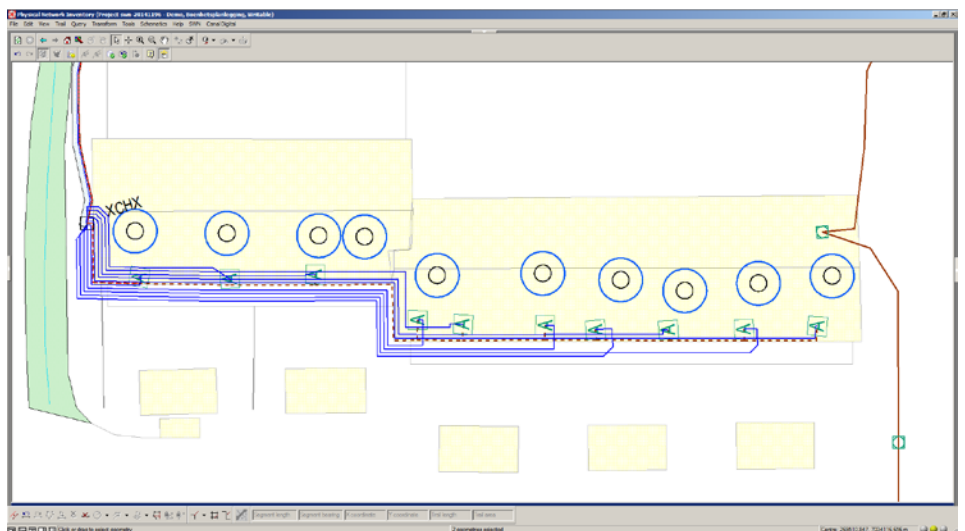
Cables and conduits in underground route section.
